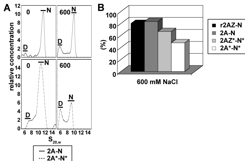
FIGURE 4: Salt-dependent stability of acetylated and nonacetylated H2A- and H2A.Z-containing NCPs. (A) Profile of analytical ultracentrifuge analysis of nucleosomes containing H2A with a non-acetylated histone complement or acetylated H2A with an acetylated histone complement at 0 and 600 mM NaCl. D: free 155 bp DNA. N: nucleosome core particle. (B) Nucleosome stability analysis of H2A or H2A.Z with non-acetylated histone complement, acetylated H2A, or acetylated H2A.Z with acetylated complement. Results show the percentage of undissociated nucleosome core particles containing a full histone octamer [calculated from the ratio (%) of area under N in panel A at a given salt level to the area under N in the absence of salt].
