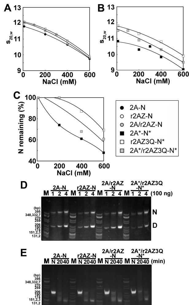
FIGURE 8: Heteromorphous H2A–H2A.Z nucleosome with a conformation and stability intermediate between those of H2A and H2A.Z homomorphous nucleosomes. (A and B) Ionic strength dependence of the sedimentation coefficient ( s_{20,w} ) of nucleosome core particles reconstituted with several constructs. Reconstituted nucleosome core particles were dialyzed against 20 mM Tris-HCl, 0.1 mM EDTA (pH 7.5) buffer containing different NaCl concentrations and analyzed by analytical ultracentrifugation at 44000 rpm and 20 °C. (C) Nucleosome stability analysis of acetylated H2A (black square), H2A.Z 3Q (white square), or an acetylated H2A/H2A.Z 3Q mixture (gray square) with acetylated complement. Results show the percentage of nucleosome core particles containing a full histone octamer. (D) Reconstituted nucleosomes run on a 4% native gel. M: Cfo I-digested pBR322 plasmid DNA as a marker. H2A; nucleosome containing H2A. H2A.Z; nucleosome containing H2A.Z. Mix: heteromorphous nucleosome containing H2A and H2A.Z. AcMix: heteromorphous nucleosome containing acetylated H2A and H2A.Z 3Q with acetylated complement. Numbers are the amounts loaded, and N and D mark the nucleosome and free DNA, respectively. (E) All nucleosomes have the same sensitivity to MNase. Lanes are the same as in panel D, and the numbers are the time of MNase treatment in minutes.
