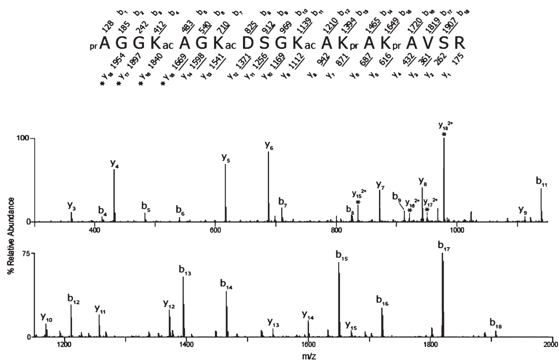
FIGURE 1: CAD MS/MS spectrum of triply acetylated H2A.Z peptide 1–19. The ion selected for dissociation was the [M + 2H]^{2+} ion ( m/z 1041.1). The amino acid sequence is shown above the spectrum, and the masses above and below the sequence correspond to the theoretical b- and y-type product ions, respectively. The masses provided are the monoisotopic, nominal masses of the product ions. The observed, singly protonated b- and y-type ions are underlined and are assigned to their corresponding m/z peaks in the spectrum. The observed, doubly protonated ions are denoted with asterisks. The acetylated lysines (K4, K7, and K11) are indicated with ac. The unacetylated amino groups were derivatized with propionic anhydride and are denoted with pr.
